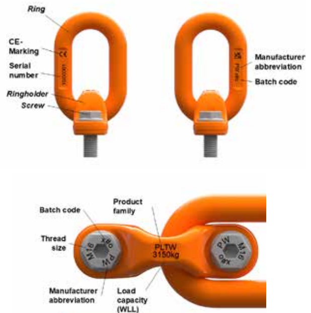
Pic. 3: Component descriptions and location of the identification details on the product.
