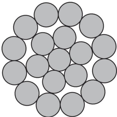
Stay rope
