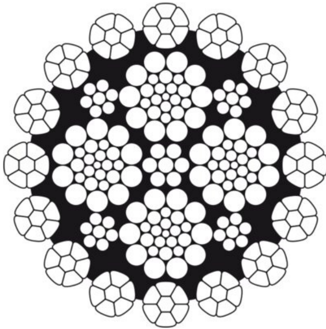
Tower crane
